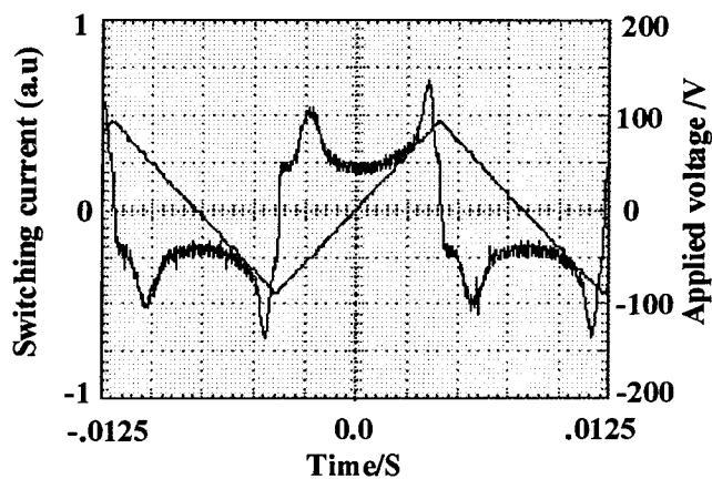
Figure 11. Switching current response in the B_2 phase of compound 20 on applying a triangular voltage ( 173\text{ V}_{\text{pp}} , 65\text{ Hz} , 105.5^\circ\text{C} ).
